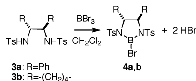
SCHEME 2. Preparation of the Chiral Lewis Acids 4a,b
