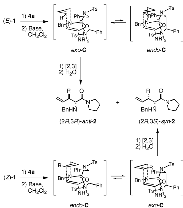
SCHEME 7. Proposed Transition States in the Kinetically Controlled Rearrangement of 1 a
