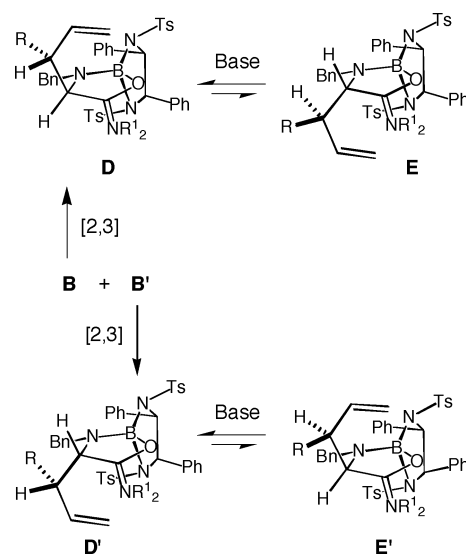
SCHEME 8. Thermodynamically Controlled Reaction Pathway a
